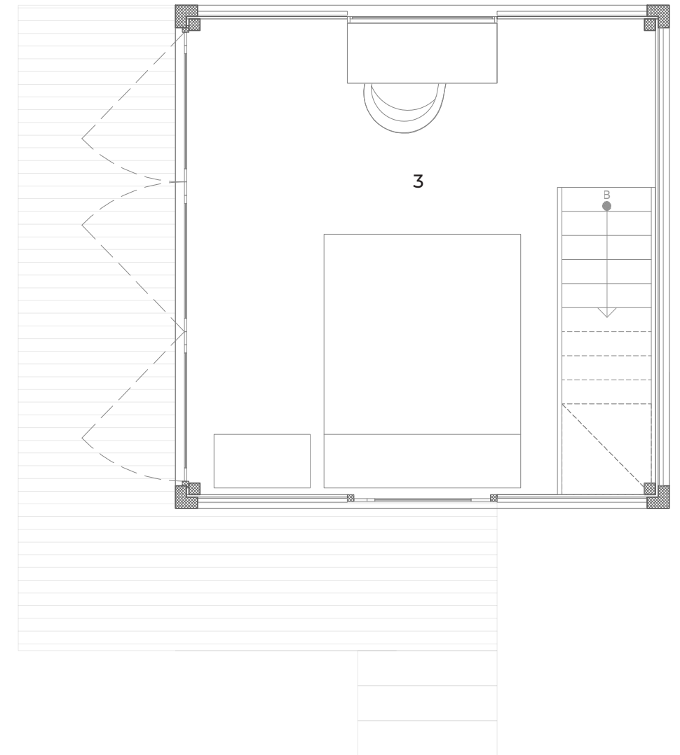
MEZZANINE
